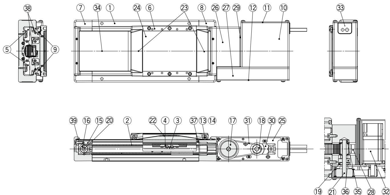
Motor details
