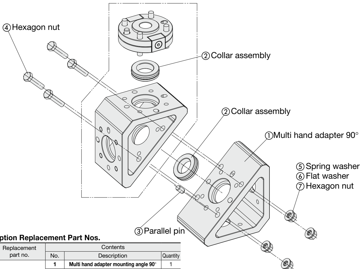
Mounting example
