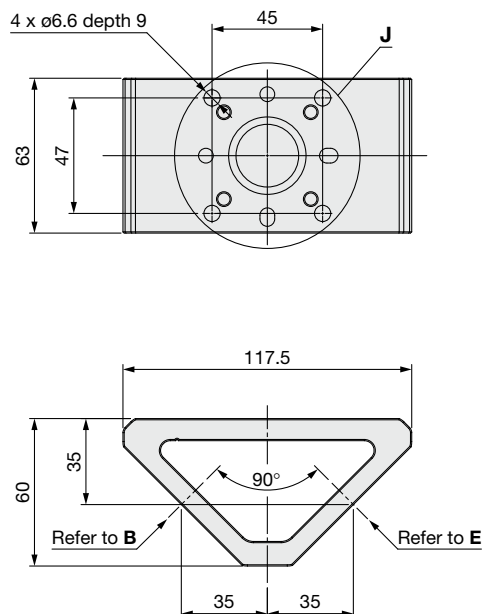
RMMA1-20T090-N: Mounting Angle 90°
