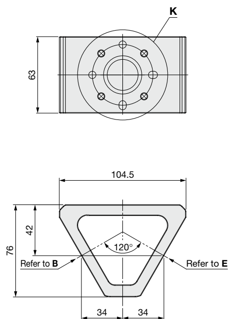
RMMA1-20T120-N: Mounting Angle 120°
